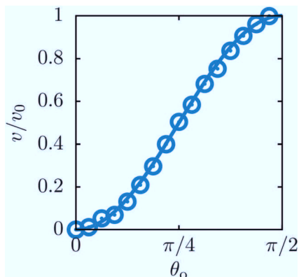
Fig. 9 The velocity v of a self-diffusiophoretic colloid as a function of the opening angle \theta_o , normalized by v_o = v(\theta_o = \pi/2) (see Fig. 5). The symbols are simulation data whereas the solid line provides the analytical prediction. 42
