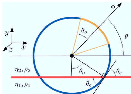
Fig. 1 Illustration of the system of a self-diffusiophoretic colloid (sphere) at a fluid–fluid interface (red, solid line) between two fluids with dynamic viscosities \eta_1 and \eta_2 and reactant mass densities \rho_1 and \rho_2 . The blue line represents the inert region of the colloid surface, while the orange, solid line represents the catalytic region with opening angle \theta_o . The colloid is partially wetted by both fluids and its position with respect to the interface is captured by the contact angle \theta_c . The orientation of the colloid with respect to the interface is characterized by the angle \theta between the axis \mathbf{o} of the colloid and a line parallel to the interface (black, solid line). Here the orientation of the particle corresponds to \theta_o > 0 .
